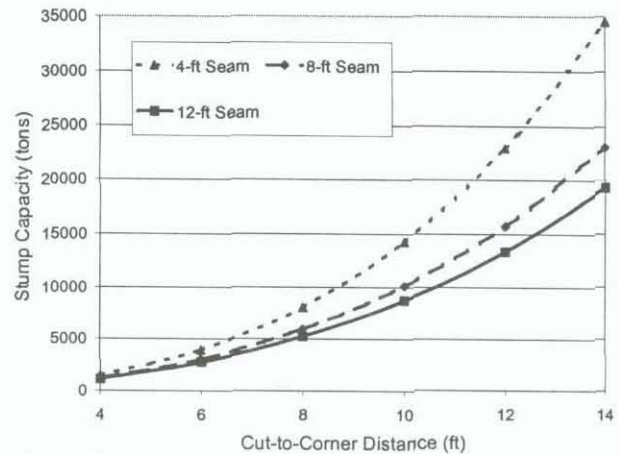
Figure 6. Load-bearing capacity of final stump for a variety of seam heights, assuming that L_1=L_2=L , \phi_1=\phi_2=75 deg., and that the stump has not yielded. An SF of 2.5 is suggested to account for yielding of the stump.
